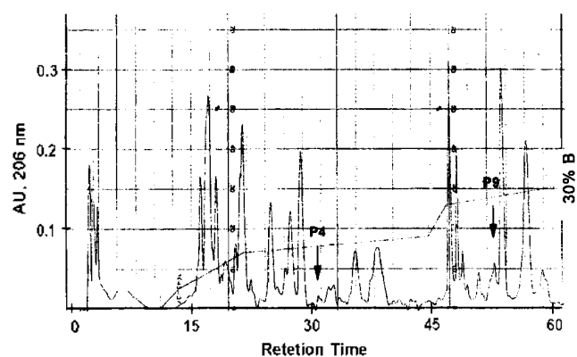
Figure 1. Tryptic digest pattern of MBP on reversed-phase C18 column chromatography. Gradient was modified for faster elution and better resolution of phosphopeptides with flow rate of 0.75 ml/min for 60 min. P4 and P9 represent two major phosphopeptides.
