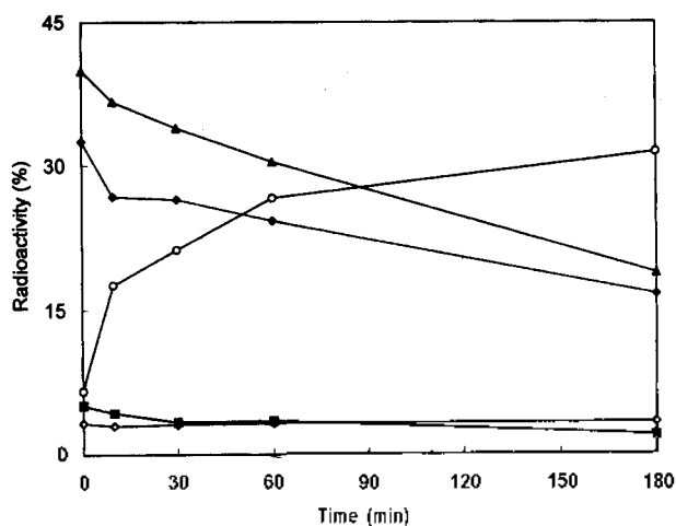
Figure 4. Time course of dephosphorylation of major peaks. [ ^{32} P]MBP was dephosphorylated by PP2B for various time periods. P0 (O), P3 (◇), P4 (●), P5 (■), P9 (▲). P0, unfettered inorganic phosphates, increased as time went by whereas others fell down.
