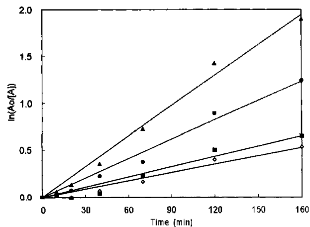
Figure 6. Logarithmic calculation of time course of dephosphorylation of [ ^{32} P]MBP by purified PP2C. [A] stands for the concentration of Ser Thr-P; A0 is the concentration of A at zero time. P0 (O), P3 (◇), P4 (●), P5 (■), P9 (▲).
