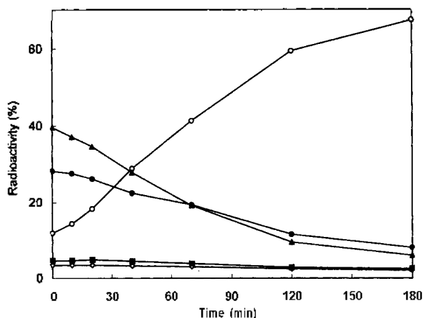
Figure 5. Time course of dephosphorylation of major peaks. [ ^{32} P]MBP was dephosphorylated by PP2C for various time periods. P0 (O), P3 (◇), P4 (●), P5 (■), P9 (▲).
