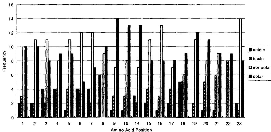
Fig. 5. Frequency and positional distribution of amino acid types in the 25 samples. The amino acid residues were divided into acidic (Asp, Glu), basic (Lys, Arg, His), nonpolar (Ala, Val, Leu, Ile, Pro, Phe, Trp, Met), and polar (Gly, Ser, Thr, Cys, Tyr, Asn, Gln) types. The total number of each amino acid type at each residue position in the samples is indicated by the specific bars. The amino acid position is numbered as follows: X_1 \cdots X_{10} \Phi G \delta X_{14} \cdots X_{23} .
