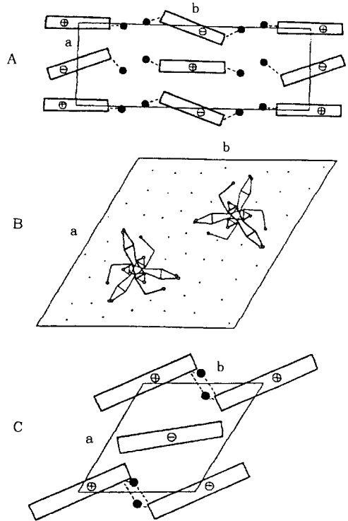
A. Na-cellulose I (filled circles indicate Na+ ions) B. Na-cellulose II B C. Na-cellulose IV (filled circles indicate water molecules)
