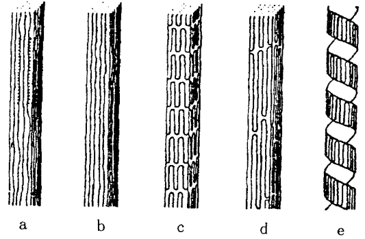
a) Fringe micell(Frey-Wyssling) b) Extended-chain model(신장쇄 모형, Hess) c) Folded chain arrangement(Dolmetsch) d) Interlinked chain conformation(Marxa-Figini) e) Tightly wound ribbon of folded chains(Manley)
