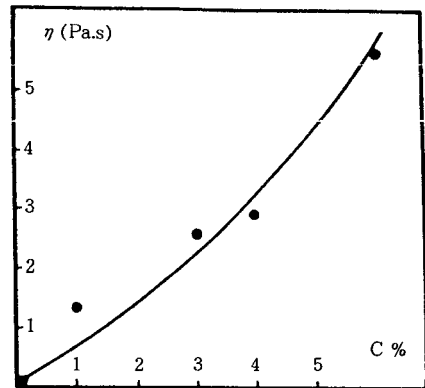
그림 1. Viscosity( \eta ) vs. concentration for solutions of cellulose (DP=600) in NMMO monohydrate at 73 °C.
