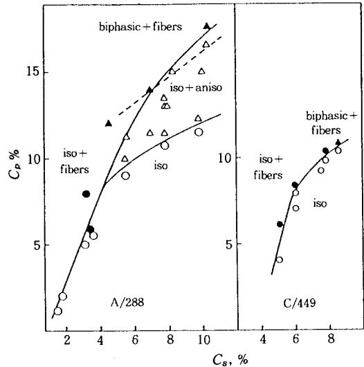
그림 7. Phase diagrams for cellulose, samples A and C, in DMAc with varying LiCl concentration at 20 °C : (○) isotropic solution; (●) isotropic solution+solid; (△) biphasic solution; (▲) biphasic solution+solid. Broken line indicates the upper limit of the biphasic gap of C_p'/C_p' \sim 1.3 .
