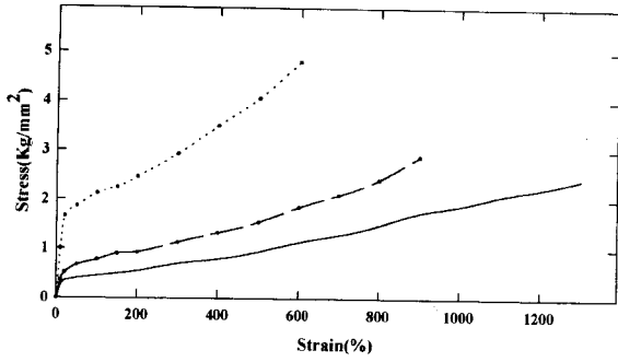
Fig. 7. Stress-strain curve of polyester type PU/PMMA hybrid with the MMA contents at 6 wt% of DMPA. --- : MMA 0 wt% —●— : MMA 20 wt% ...○... : MMA 40 wt%
