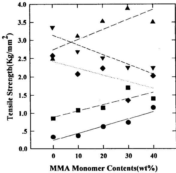
Fig. 5. Tensile strength of polyester type PU/PMMA hybrids with the MMA contents. ● : DMPA 2 wt% ■ : 4 wt% ▲ : 6 wt% ▼ : 8 wt% ◆ : 10 wt%
