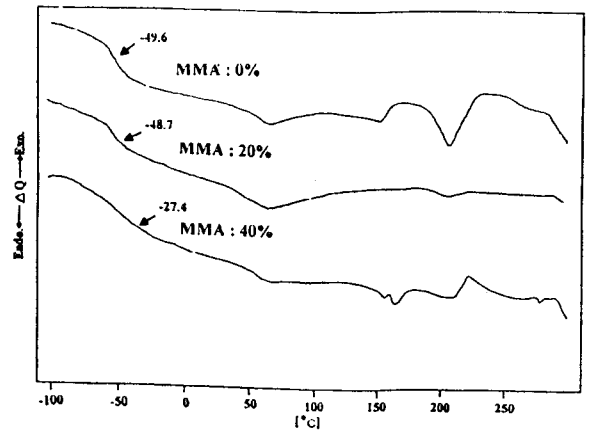
Fig. 11. DSC thermograms of polyester type PU/PMMA hybrid with the MMA contents at 6 wt% of DMPA.
