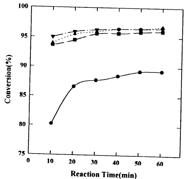
Fig. 4. The conversion of PU/PMMA hybrids with the PUD ionic contents.
