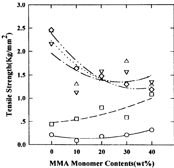
Fig. 6. Tensile strength of polyether type PU/PMMA hybrids with the MMA contents. ○ : DMPA 2 wt% □ : 4 wt% △ : 6 wt% ▽ : 8 wt% ◇ : 10 wt%
