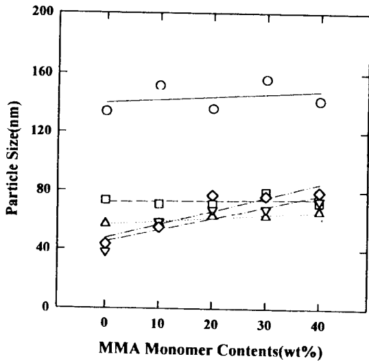
Fig. 3. The particle size of polyester type PU/PMMA hybrid with different DMPA contents.
