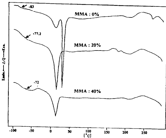
Fig. 9. DSC thermograms of polyether type PU/PMMA hybrid with the MMA contents at 2 wt% of DMPA.
