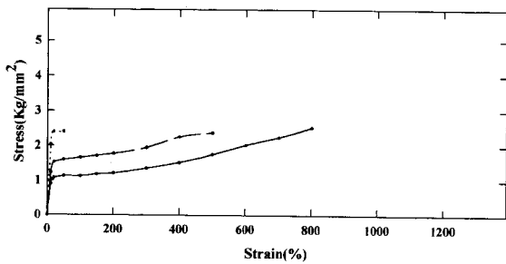
Fig. 8. Stress-strain curve of polyester type PU/PMMA hybrid with the MMA contents at 8 wt% of DMPA. --- : MMA 0 wt% —●— : MMA 20 wt% ...○... : MMA 40 wt%
