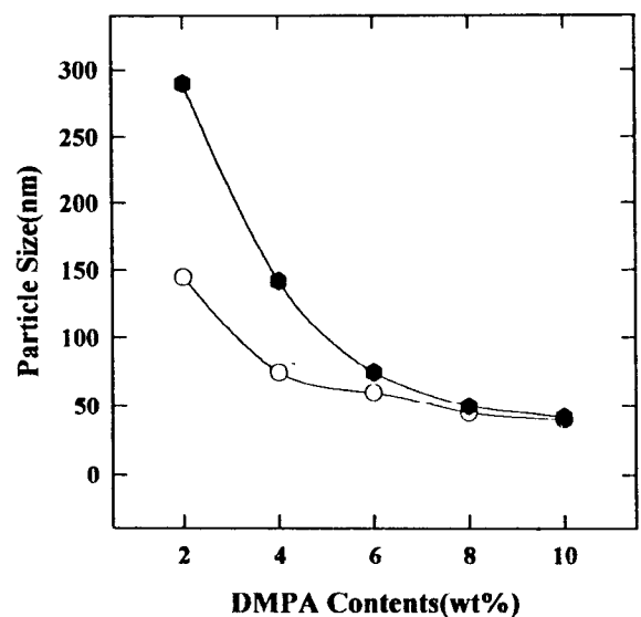
Fig. 1. The particle size change with different polyols.
