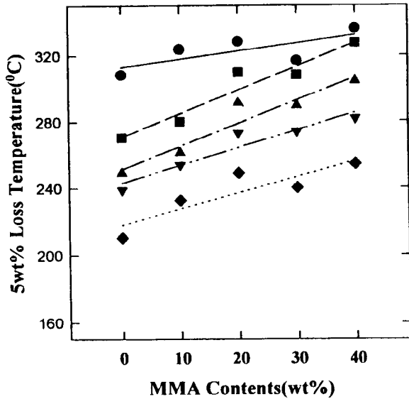
Fig. 12. 5 wt% loss temperature of polyester type PU/PMMA hybrid with the ionic group and MMA contents. -●- : DMPA 2 wt% -■- : 4 wt% -▲- : 6 wt% -▼- : 8 wt% -◆- : 10 wt%
