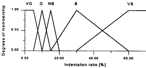
(b) Indentation ratio membership function for indentation output
