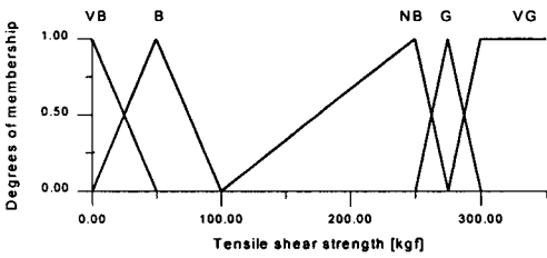
(a) Tensile shear strength membership function for strength output
