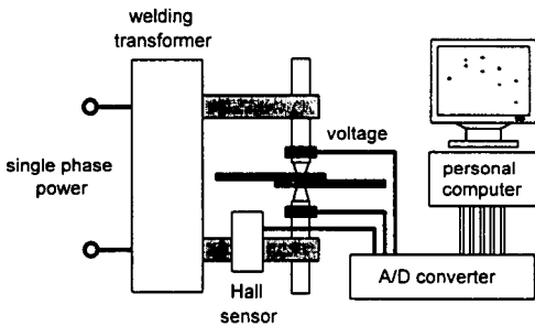
Fig. 1 Schematic diagram of welding variable measurement system
