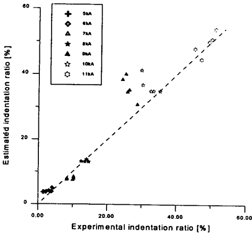
Fig. 13 Correlation of indentation ratio between estimated and experimental result
