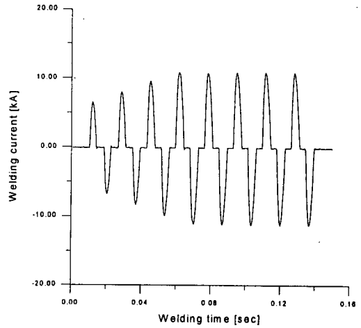
(a) Current=6kA
