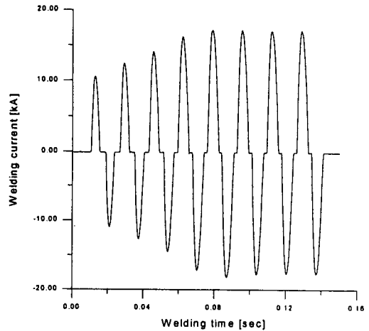
(b) Current=11kA
