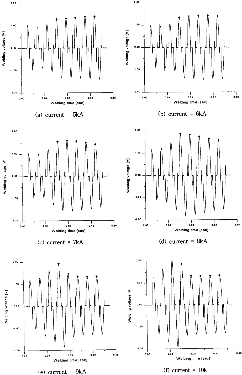
Fig. 3 Waveform of measured welding voltage for various welding current (Welding time : 8 cycle, electrode force:250kgf)
