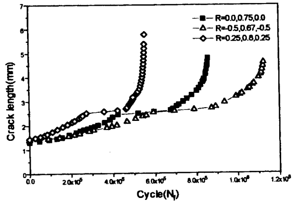
Fig. 9 Relation between crack length( a ) and cycle( N_f )
