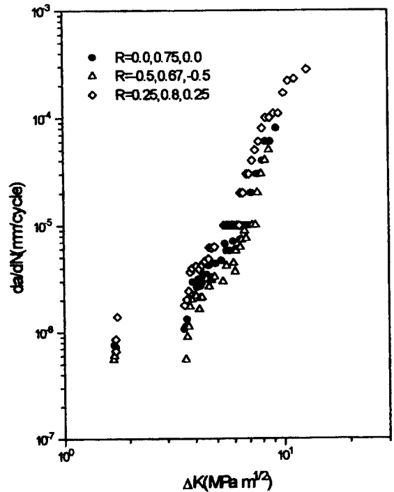
Fig. 4 The fatigue crack growth rate ( da/dN ) vs. the stress intensity factor range ( \Delta K )
