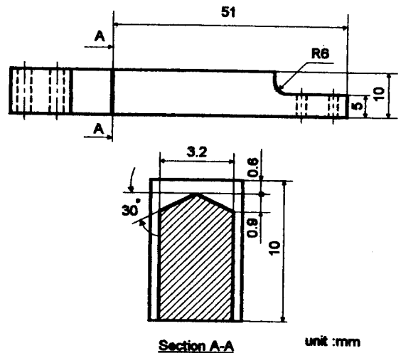
Fig. 1 Configuration of test specimen
