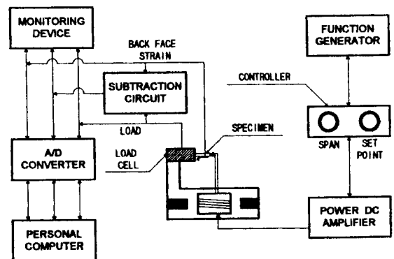
Fig. 3 System of fatigue test
