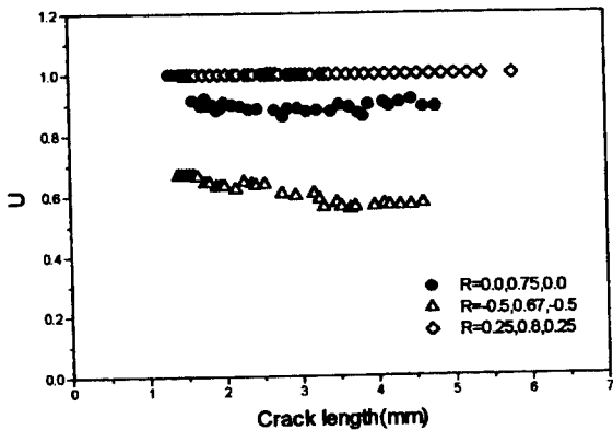
Fig. 8 Relation between effective stress intensity factor range ratio( U ) and crack length( a )
