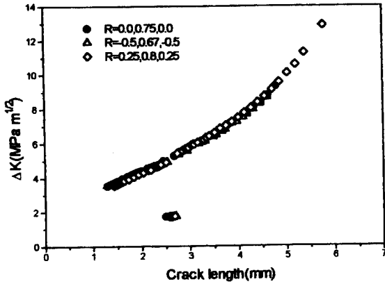
Fig. 6 Relation between stress intensity factor range( \Delta K ) and crack length( a )
