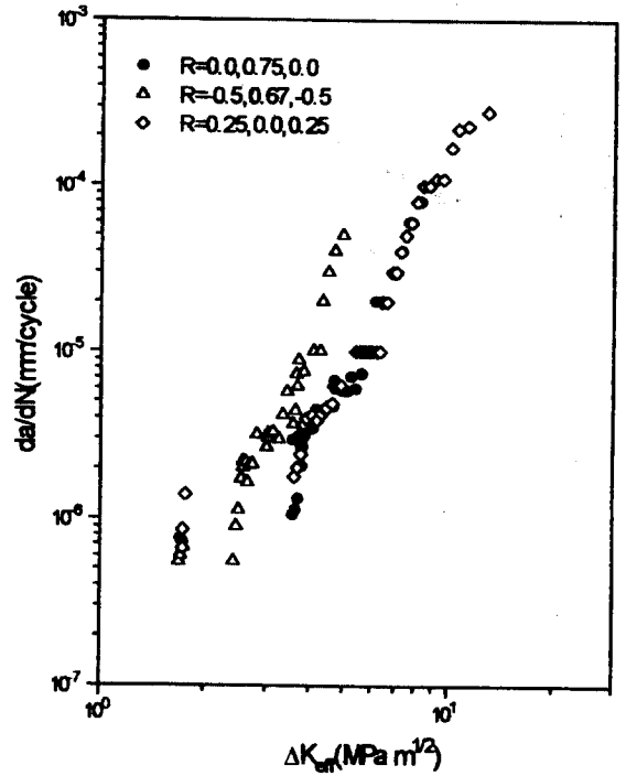
Fig. 5 The fatigue crack growth rate( da/dN ) vs. the effective stress intensity factor range( \Delta K_{eff} )
