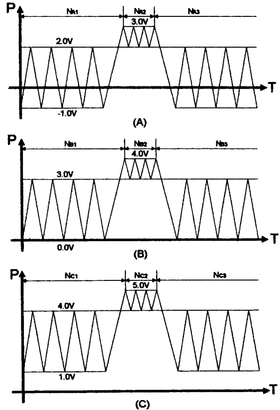
Fig. 2 Load patterns
