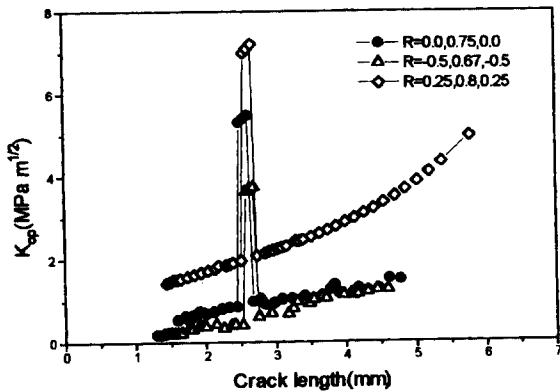
Fig. 7 Relation between stress intensity factor at crack opening point( K_{op} ) and crack length( a )
