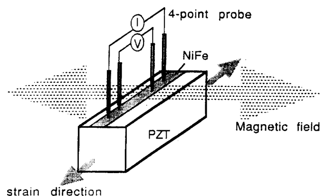
Fig. 1. Experimental setup.
