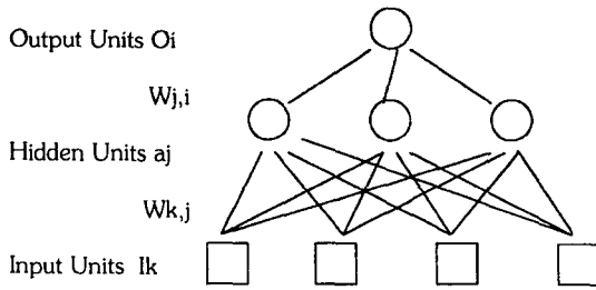
Fig. 1. A Tow-layer Feed Forward Network.
