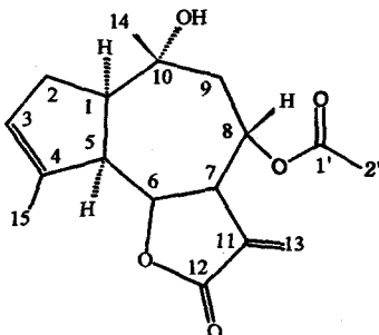
Fig. 2. Chemical structure of cumambirin A.
