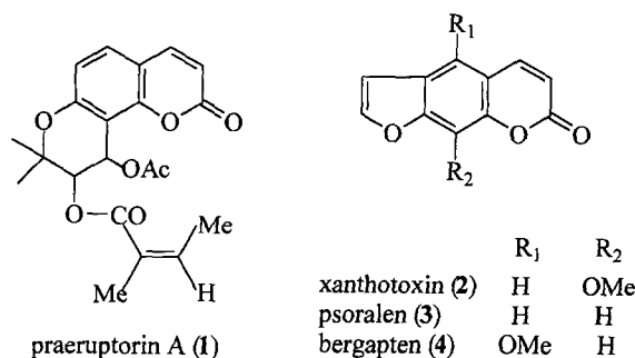
Fig. 1. Structures of compounds isolated from P. japonicum .
