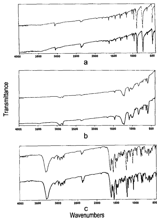
Fig. 3. IR absorption spectra of the chemicals. a: anthracene, b: sodium lauryl sulfate, c: melatonin. Upper spectra: irradiation, lower spectra: non-irradiation.
