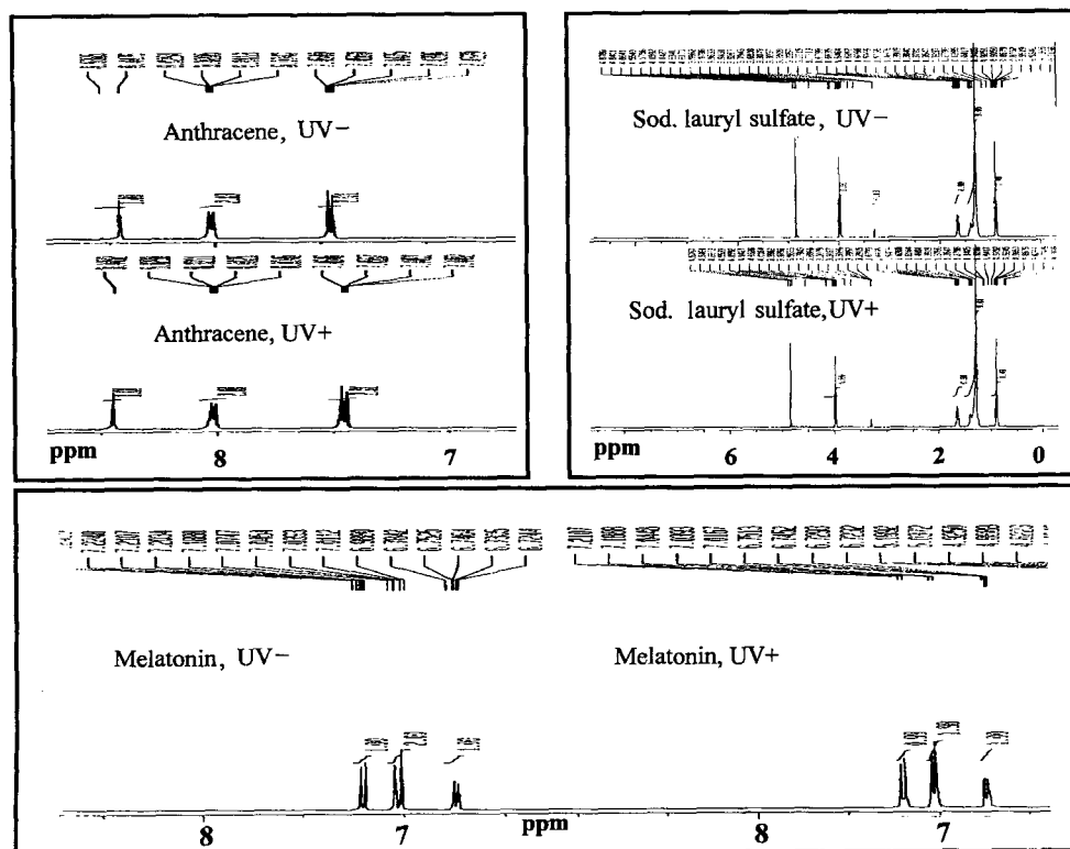
Fig. 4. 1 H-NMR spectra of the chemicals.
