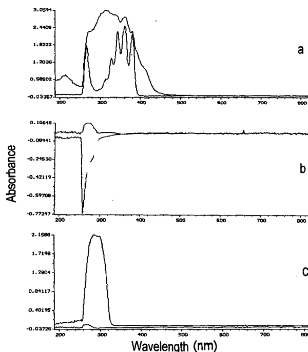
Fig. 2. Ultraviolet absorption spectra of the chemicals. a: anthracene, b: sodium lauryl sulfate, c: melatonin. Upper spectra: irradiation, lower spectra: non-irradiation.
