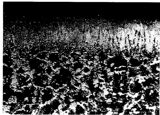
Photo. 2 Optical microstructure of the boride layer on SM45C obtained by the modified boronizing process, which was first treated at 650℃ for 1hr and then treated at 800℃ for 7hrs, respectively, in 1.5vol.%BCl 3 -50vol.%H 2 -Ar mixed gas with 266Pa.
