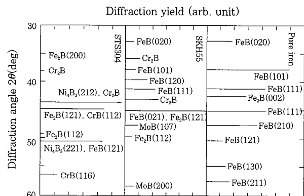
Fig. 3 XRD patterns of glow discharge boronized pure Fe, SKH 55 and STS 304 at 700℃ for 1h 11) .
