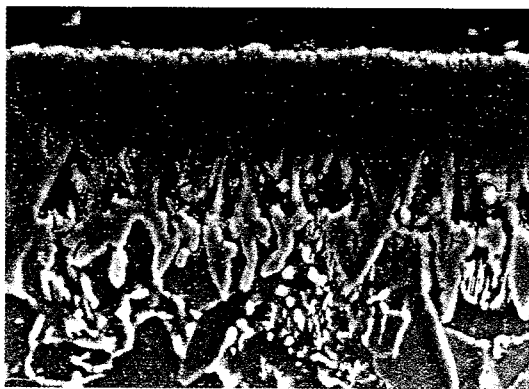
Photo. 1 SEM micrograph of the boride layer on SM45C, which was formed at 800℃ for 4hrs in 3vol.%BCl 3 -30vol.%H 2 -Ar mixed gas with 665Pa.
