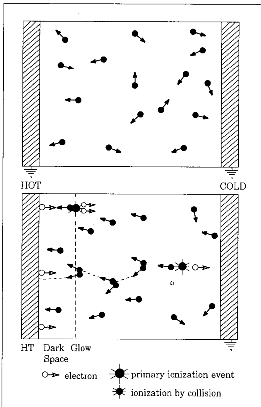
Fig. 1 Schematic diagram showing essential differences in molecular motion between (a)gaseous and (b)plasma treatment 1)
