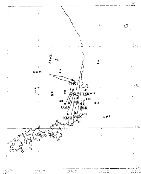
Fig. 1 Study area in the Kyeongsang Basin. Triangles represent seismograph stations, and solid circles represent earthquakes used in this study
