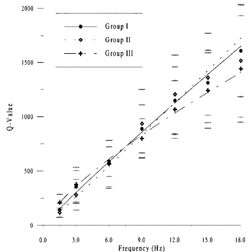
Fig. 2 Summary of results for coda Q values with frequencies. Each 3 curve indicates the best fitting by linear regression. Numerical results are summarized in Table 2 and Table 3.
