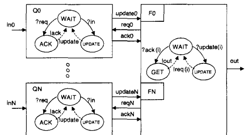
Fig. 5. Model of an N-input Multiplexer
