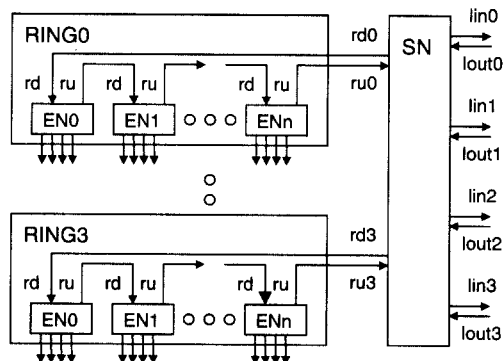
Fig. 2. System Architecture
