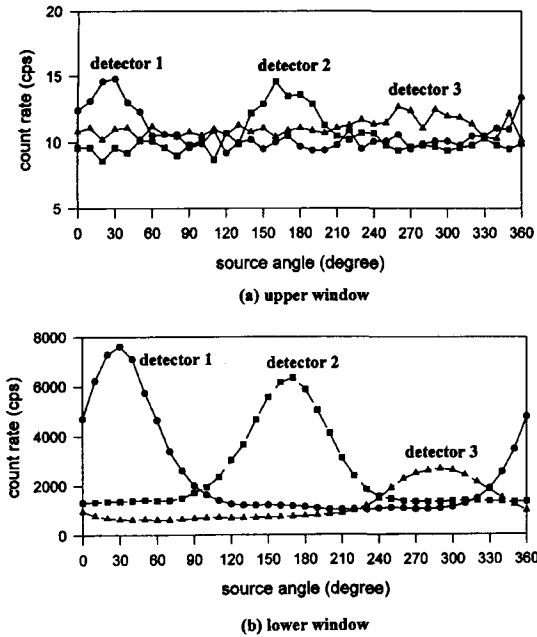
Fig. 3. Reference Responses for 2nd Ring Labeled with 192 Ir. (The rough peaks at the upper window are due to coincidence sum effect.)
