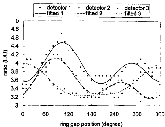
Fig. 9. Ratio of Counts Measured in Lower Window to in Upper Window for Top Ring( 60 Co)
