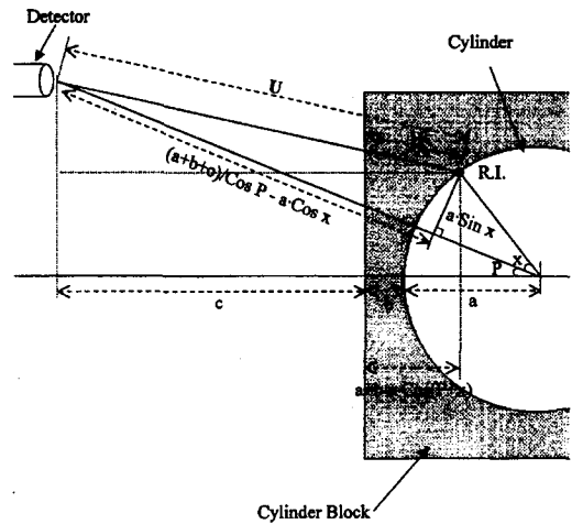
Fig. 4. Geometrical Model of Experiment for Obtaining Calibration Functions
