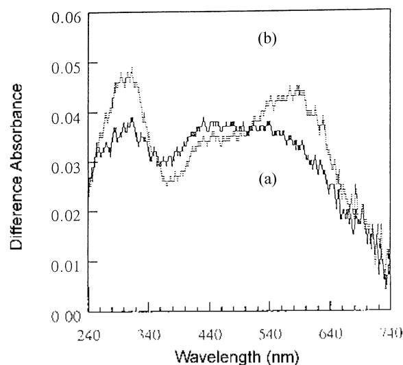
Figure 3. The difference spectra between the reduced and neutral states of the tbcCuPc adsorbed on PGE at -650 mV(a) and -760 mV(b), respectively.
