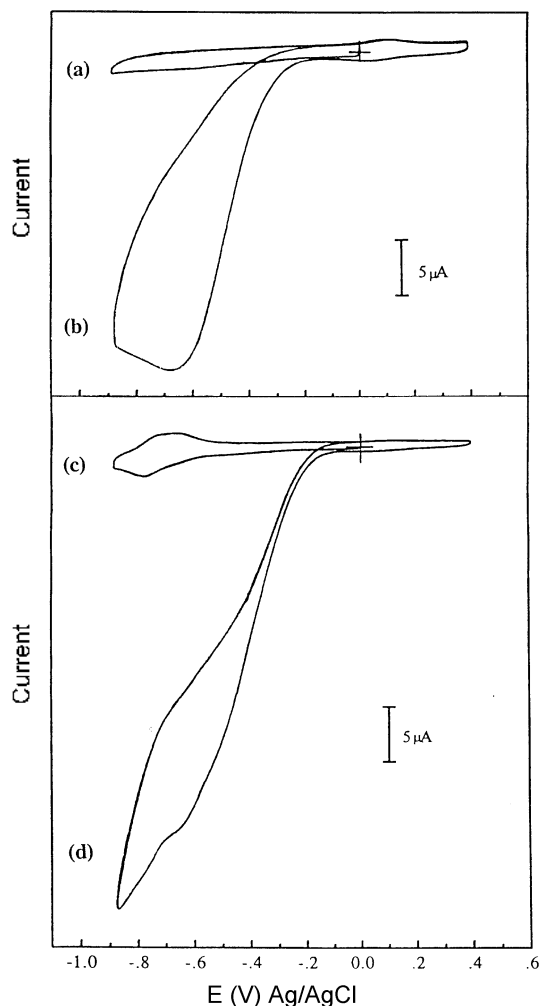
Figure 4. CVs recorded for the reduction of O_2 with (a) bare PGE in an argon gas purged phosphate buffer solution. (b) bare PGE in an air saturated buffer solution. (c) tbcCuPc adsorbed PGE in the argon gas purged buffer solution. and (d) tbcCuPc adsorbed PGE in the air saturated buffer solution. The scan rate was 100 mV/s.
