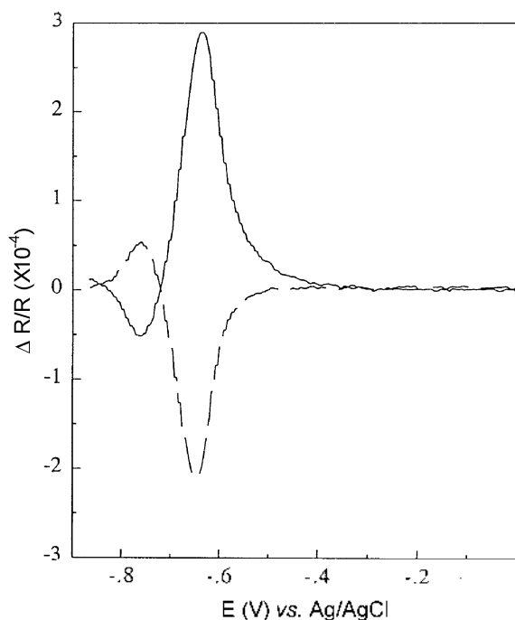
Figure 2. ER voltammogram of the tbcCuPc adsorbed on PGE in the phosphate buffer solution (pH 7.04) recorded at 600 nm, f = 14 Hz, and \Delta E_{ac} = 30.65 mV with scan rate of 2 mV/sec. The solid and dashed lines indicate real and imaginary parts, respectively.
