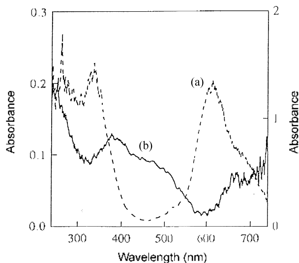
Figure 1. UV-Vis. spectra for (a) 1.0 \times 10^{-4} M tbcCuPc in chloroform and (b) adsorbed tbcCuPc on PGE in a phosphate buffer solution (pH=7.04).
