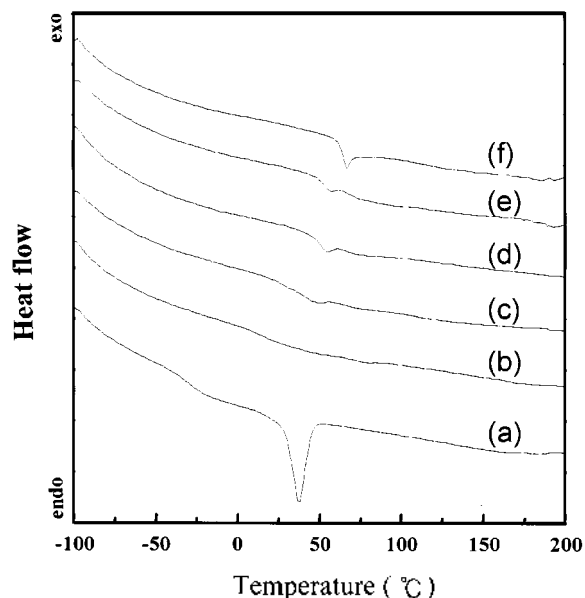
Figure 3. DSC thermograms for blends of CPU/CPVC: (a) 100/0, (b) 80/20, (c) 60/40, (d) 40/60, (e) 20/80, and (f) 0/100.
