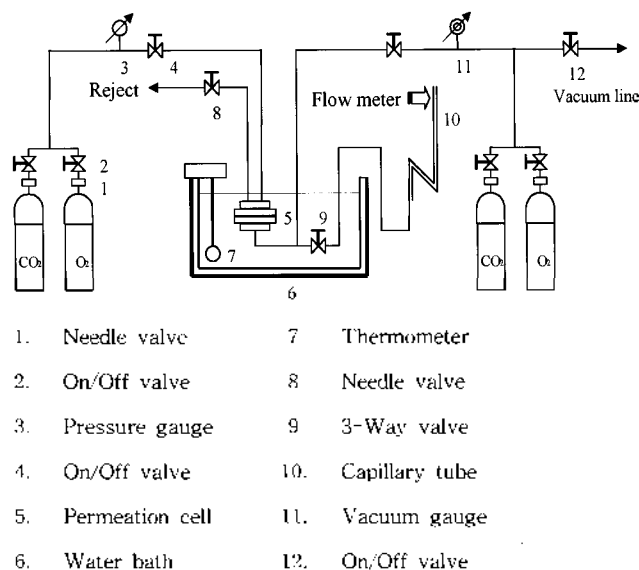
Figure 1. The experimental apparatus for permeability measurement.
