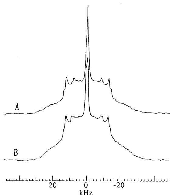
Figure 3. ^2\text{H} NMR spectra of the bilayers of the mixture of E. coli phosphatidylethanolamine (EPE) and 1,2-dimyristoyl- sn -glycero-3-phosphoethanolamine (DMPE) at 55 °C. Mixing ratio is one to one (w/w). (A) deuterated EPE and nondeuterated DMPE. (B) deuterated EPE and deuterated DMPE. The doublets appear at about 8 kHz.
