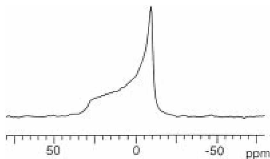
Figure 2. A ^{31}\text{P} NMR spectrum of deuterated E. coli phosphatidylethanolamine bilayers at 55 °C under proton-decoupling.
