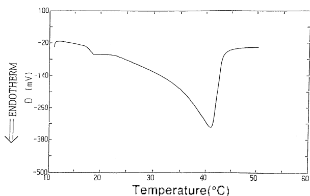
Figure 5. Thermogram of differential scanning calorimetry of (1,2-dimyristoyl- sn -glycerol-3-phosphoethanolamine + E. coli phosphatidylethanolamine) bilayers (1 : 1, w/w).
