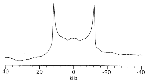
Figure 4. ^2\text{H} NMR spectrum of E. coli phosphatidylethanolamine bilayers at 50 °C specifically deuterated at the C2 position of the glycerol backbone.
