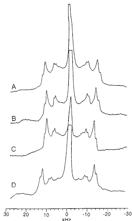
Figure 6. ^2\text{H} NMR spectra of the deuterated E. coli phosphatidylethanolamine (EPE*) mixed with other nondeuterated phospholipids in the liquid-crystalline state (at 50 °C). The glycerol backbone is perdeuterated. Mixing ratio is one to one (w/w). (A) EPE*. (B) EPE* + E. coli phosphatidylglycerol. (C) EPE* + E. coli cardiolipin. (D) EPE* + 1,2-dipalmitoyl- sn -glycerol-3-phosphocholine (DPPC).
