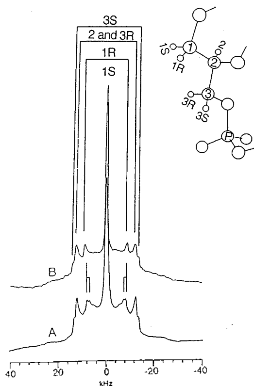
Figure 1. 2 H NMR spectrum of E. coli phosphatidylethanolamine bilayers at 50 °C (A) and 1,2-dipalmitoyl- sn -glycero-3-phosphoethanolamine (DPPF) bilayers at 75 °C (B) perdeuterated in the glycerol backbone. Assignments are given on the top along with the structural description.
