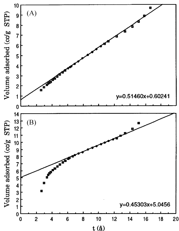
Figure 6. A t -plot calculated from the isotherm obtained from CM-MgO before the second cycle treatment (A). After the second cycle treatment, the t -plot (B) showed that surface characteristics were largely modified.
