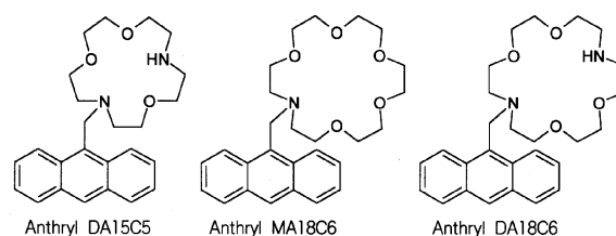
Figure 1. Structures of the synthesized Anthrylazacrown ethers.
