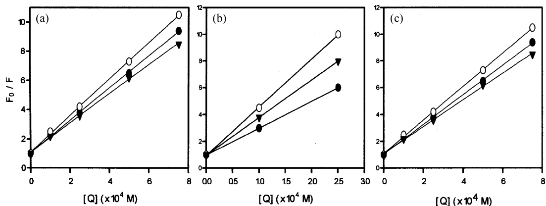
Figure 4. Stern-Volmer plotting for anthrylazacrown ethers in quenching with (a) Mn(II), (b) Co(II), and (c) Cu(II). (● : Anthryl DA15C5, ○ : Anthryl MA18C6, ▼ : Anthryl DA18C6)
