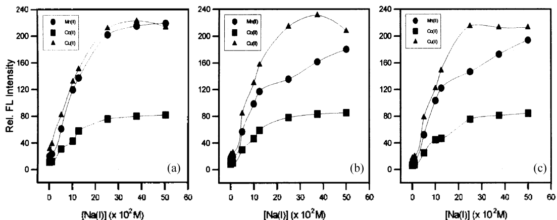
Figure 6. Enhanced fluorescence intensities in quenched anthrylazacrown ethers by Mn(II), Co(II) and Cu(II) with the concentration of added sodium nitrate; (a) Anthryl DA15C5, (b) Anthryl MA18C6, (c) Anthryl DA18C6. All solution were mixed with [anthrylazacrown ethers] 1.0 \times 10^{-7} M and [M] 5.0 \times 10^{-4} M. (M: Mn(II), Co(II), Cu(II)). Excitation was at 254 nm and emission maximum centered near 412 nm.
