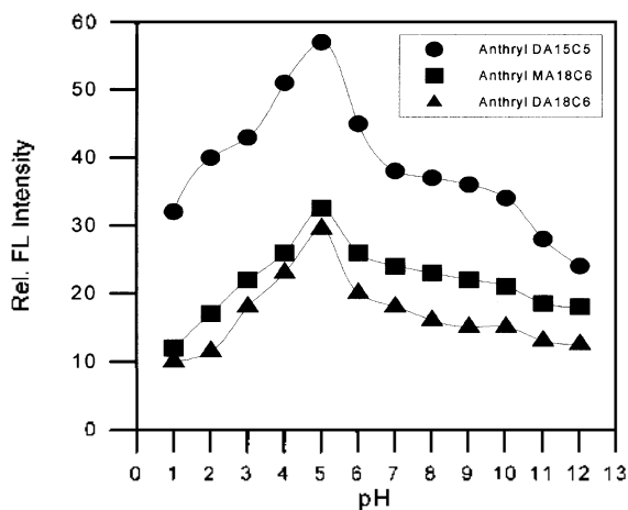
Figure 3. pH-fluorescence profiles for 0.1 \mu\text{M} solutions of Anthrylazacrown ethers. Excitation was at 254 nm; Emission was measured at the emission maximum centered near 412 nm. pHs were maintained using the following solutions; 0.2 M HCl (pH 1 and 2), 0.2 M Sodium acetate (pH 3, 4, 5 and 6), 0.2 M Tris (pH 7, 8 and 9), 0.2 M \text{NaHCO}_3 (pH 10 and 11), 0.2 M NaOH (pH 12).
