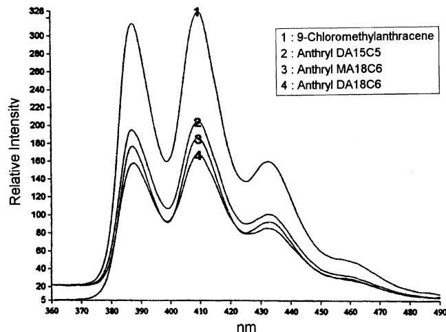
Figure 2. Relative fluorescence intensity changes for Anthrylazacrown ethers in MeOH solution.
