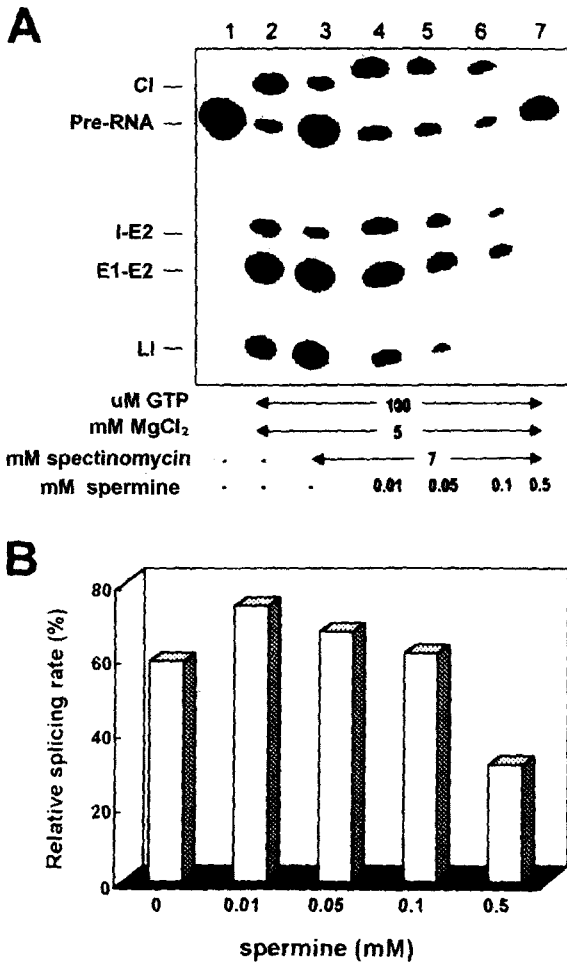
Fig. 4. Effect of spermine on the self-splicing inhibition of td intron RNA by spectinomycin. A. Autoradiogram showing the effect of varying concentrations of spermine (0.01-0.5 mM) on self-splicing in the presence of 7 mM spectinomycin. Lane 1, unspliced pre-RNA; I-E2, intron-exon 2; E1-E2, exon 1-exon 2 ligation product; LI, linear intron. B. Splicing rates of the intron RNA as a function of concentrations of spermine. The ratio of E1-E2 ligation produced in each splicing reaction to that of the normal splicing reaction was expressed as relative splicing activity.
