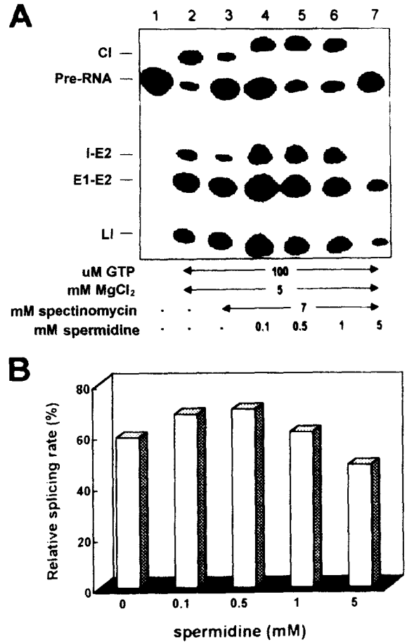
Fig. 3. Effect of spermidine on the self-splicing inhibition of td intron RNA by spectinomycin. A. Autoradiogram showing the effect of varying concentrations of spermidine (0.1-5 mM) on self-splicing in the presence of 7 mM spectinomycin. Lane 1, unspliced pre-RNA; I-E2, intron-exon 2; E1-E2, exon 1-exon 2 ligation product; LI, linear intron. B. Splicing rates of the intron RNA as a function of concentrations of spermidine. The ratio of E1-E2 ligation produced in each splicing reaction to that of the normal splicing reaction was expressed as relative splicing activity.
