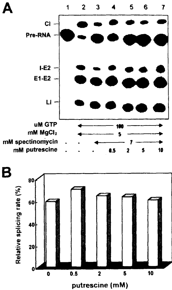
Fig. 2. Effect of putrescine on the self-splicing inhibition of td intron RNA by spectinomycin. A. Autoradiogram showing the effect of varying concentrations of putrescine (0.5-10 mM) on self-splicing in the presence of 7 mM spectinomycin. Lane 1, unspliced pre-RNA; I-E2, intron-exon 2; E1-E2, exon 1-exon 2 ligation product; LI, linear intron. B. Splicing rates of the intron RNA as a function of concentrations of putrescine. The ratio of E1-E2 ligation produced in each splicing reaction to that of the normal splicing reaction was expressed as relative splicing activity.
