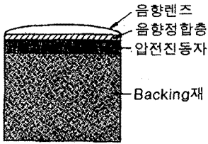
Fig. 1. Basic structure of the ultrasonic probe
