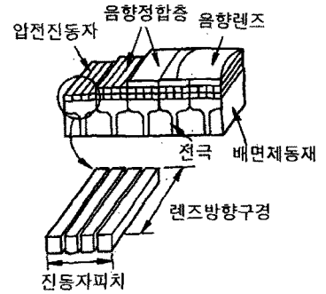
Fig. 3. Vibrator structure of the linear array probe
