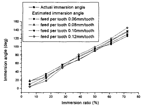
Fig. 14 Estimation of immersion angle with various immersion ratio (various feed per tooth)
