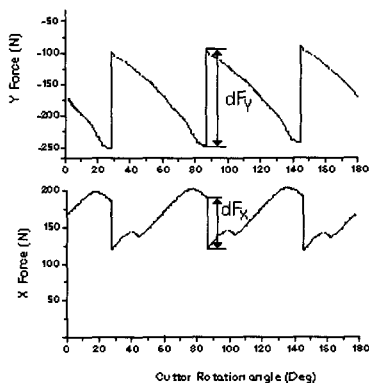
Fig. 1 Cutting force pattern when more than two teeth are involved in cutting
