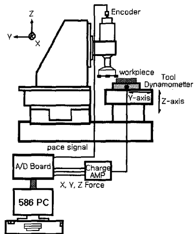
Fig. 2 Experimental set up
