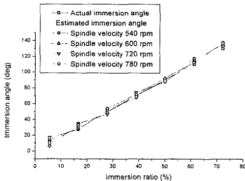
Fig. 13 Estimation of immersion angle with various immersion ratio (various spindle speed)
