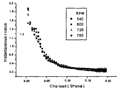
Fig. 7 Instantaneous r value with various spindle speed (feed per tooth 0.2mm/tooth, axial depth of cut 1.0mm)
