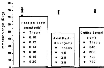
Fig. 10 Estimation of Immersion angle with various cutting condition
