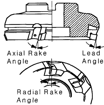
Fig. 3 Configuration of the Facemill Cutter
