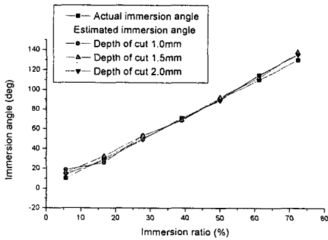
Fig. 12 Estimation of immersion angle with various immersion ratio (various axial depth of cut)
