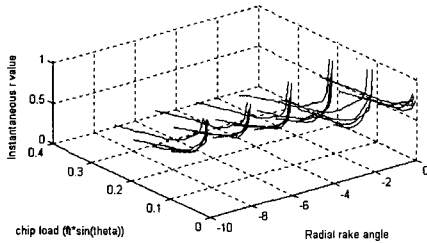
Fig. 8 Instantaneous r value with various radial rake angle (radial rake angle 0°, -2°, -4°, -6°, -8°, -10°)
