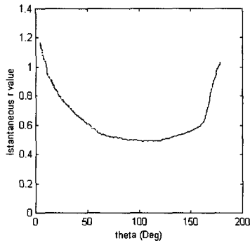
Fig. 4 Instantaneous r value at the swept angle of cut ( single tooth, feed per tooth 0.2mm/tooth, spindle speed 600rpm, axial depth of cut 2.0mm)
