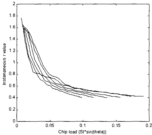
Fig. 5 Instantaneous r value with various feed per tooth (feed/tooth 0.1, 0.12, 0.14, 0.16, 0.18, 0.2 mm/tooth, spindle speed 600rpm, axial depth of cut 1.0 mm)
