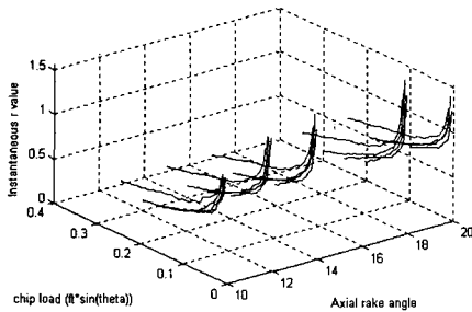
Fig. 9 Instantaneous r value with various axial rake angle (axial rake angle 10°, 12°, 14°, 16°, 18°, 20°)
