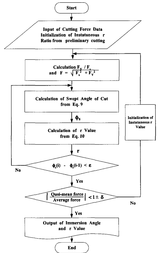
Fig. 11 Flow chart for the estimation of immersion angle
