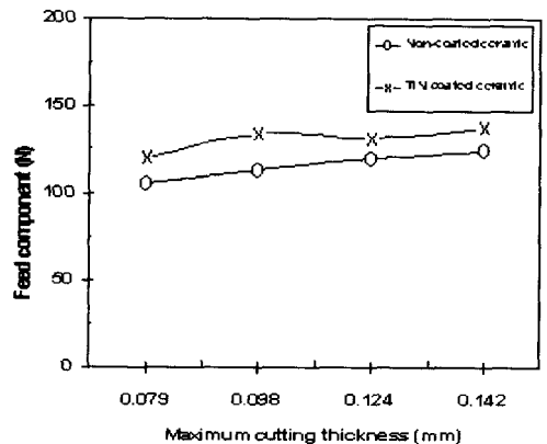
Fig. 13 Feed component with maximum cutting thickness
