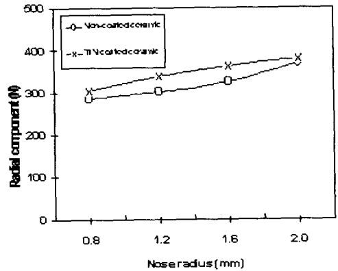
Fig. 18 Radial component with nose radius
