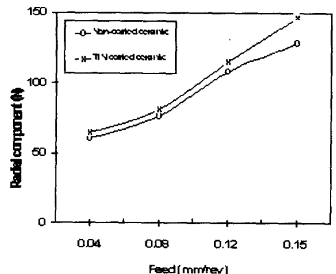
Fig. 9 Radial component with feed
