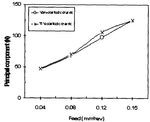
Fig. 8 Principal component with feed
