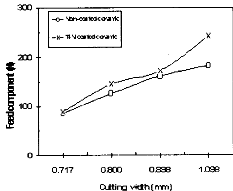
Fig. 16 Feed component with cutting width
