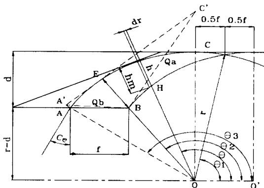
Fig. 1 Geometry of cutting cross-section or chip flow model for nose radius tool
