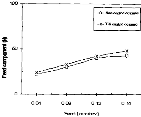
Fig. 10 Feed component with feed
