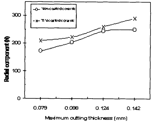
Fig. 12 Radial component with maximum cutting thickness
