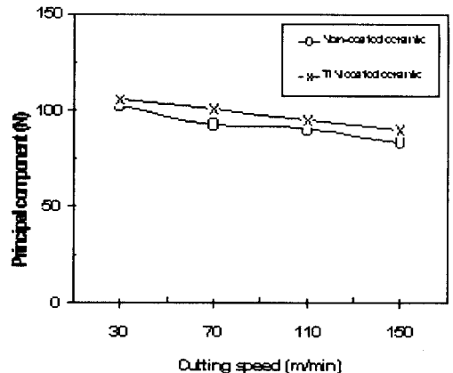
Fig. 5 Principal component with cutting speed
