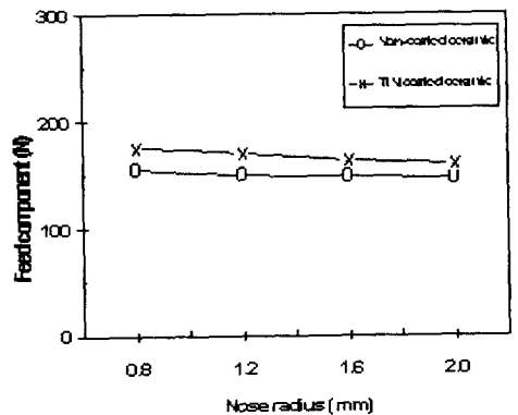
Fig. 19 Feed component with nose radius
