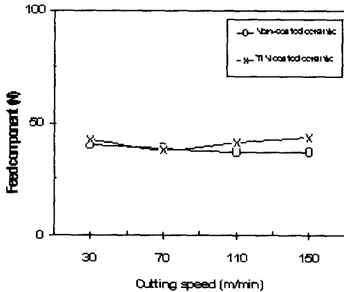
Fig. 7 Feed component with cutting speed
