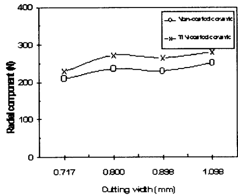
Fig. 15 Radial component with cutting width
