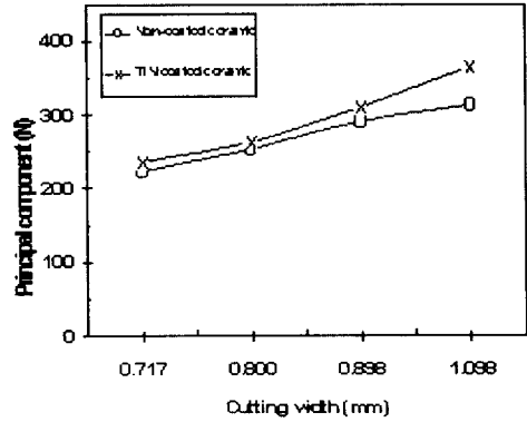
Fig. 14 Principal component with cutting width
