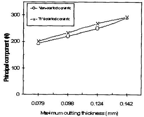
Fig. 11 Principal component with maximum cutting thickness
