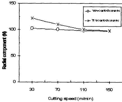
Fig. 6 Radial component with cutting speed
