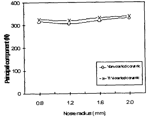
Fig. 17 Principal component with nose radius
