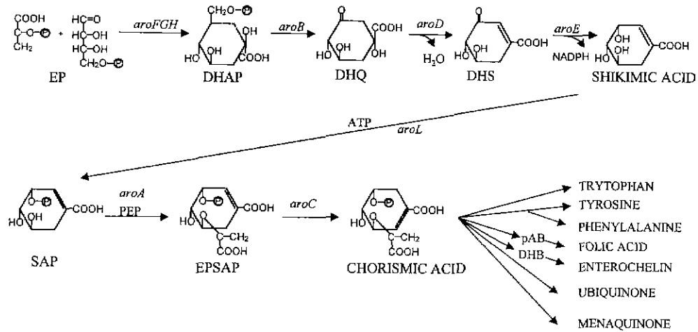
Fig. 1. Aromatic amino acid biosynthesis pathway. pAB, p-aminobenzoic acid; DHB, 2,3-dihydroxybenzoic acid; PEP, phosphoenolpyruvate; EP, D-erythrose 4-phosphate; DAHP, 3-deoxyarabinoheptulosonic acid-7-phosphate; DHQ, 5-dehydroquinate; DHS, 3-dehydroshikimate; SAP, shikimate acid 3-phosphate; EPSAP, 3-enolpyruvyl-shikimate-5-phosphate.
