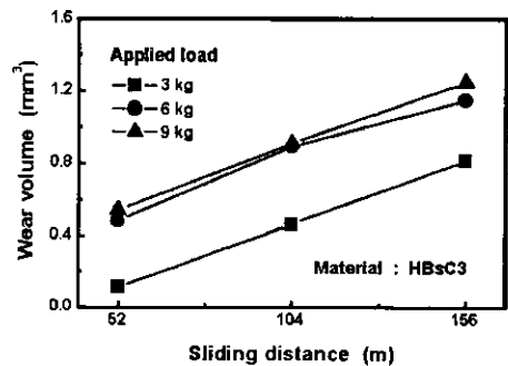
Fig. 11 Effect of sliding distance on wear volume
