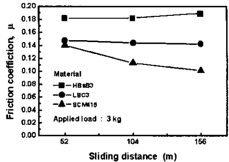
Fig. 7 Friction coefficient for specimens
