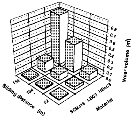
Fig. 12 Wear volumes for specimen
