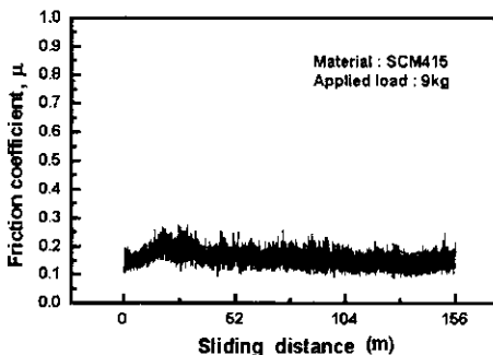
Fig. 6 Relation between friction coefficient and sliding distance
