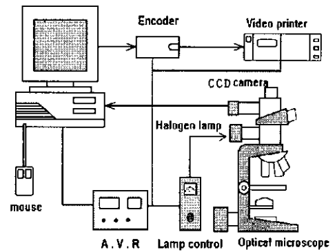
Fig. 4 Image processing system
