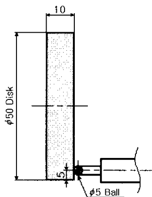
Fig. 2 Shape and dimensions of specimen
