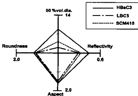
Fig. 9 Diagram of shape parameters
