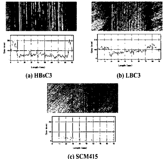
Fig. 8 Track and gray level of rubbed surface
