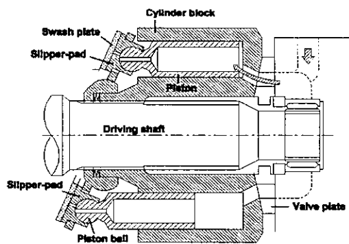
Fig. 1 Hydraulic piston motor
