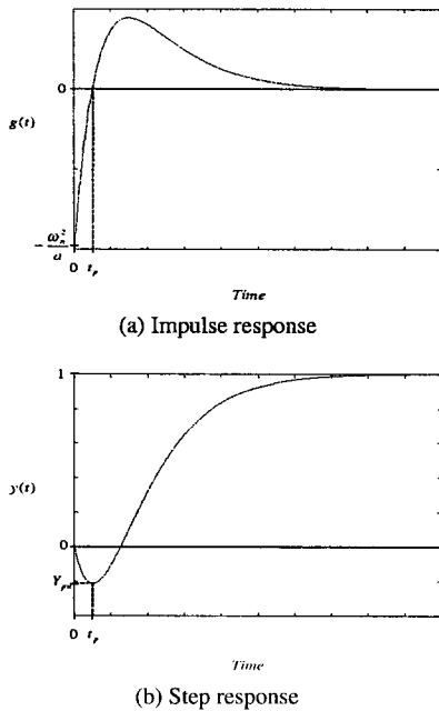
Fig.3. Impulse response and step response of critically damped case.
