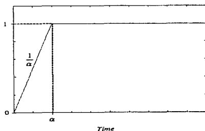
Fig.5. The compensator response to the unit step input.
