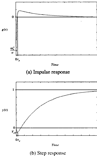
Fig.4. Impulse response and step response of overdamped case.
