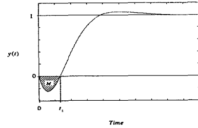
Fig.6. M and t_z in the unit step response.
