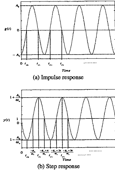
Fig. 2. Impulse response and step response of undamped system.
