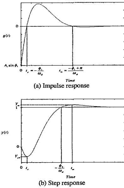
Fig. 1. Impulse response and step response of underdamped system.
