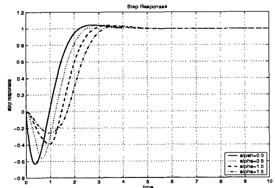
Fig.7. Step responses.
