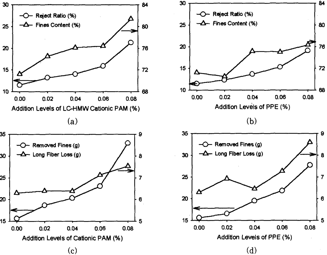
Fig. 6. The comparison of cationic PAM and PPE as a fraction promoter.
