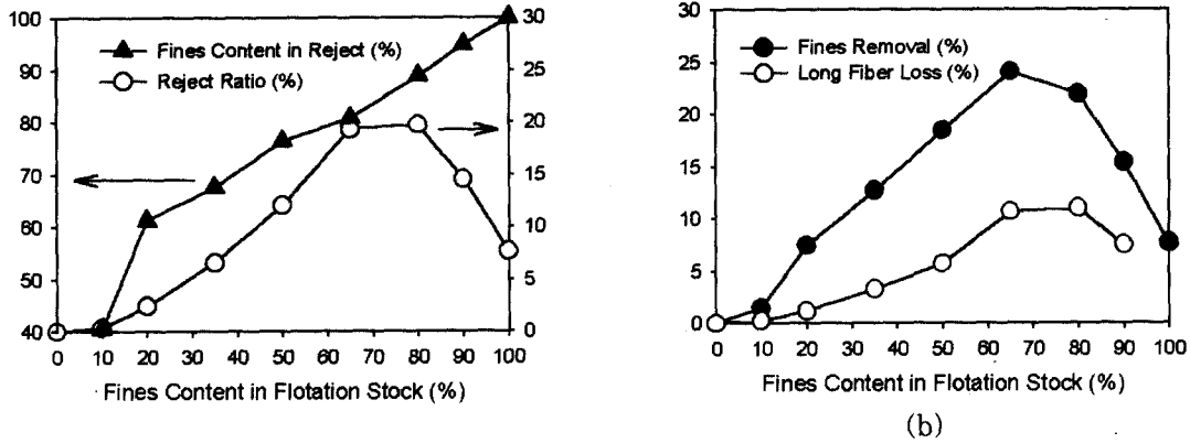
Fig. 1. The efficiency of fines fractionation in an aspect of fines contents in OCC stock.
