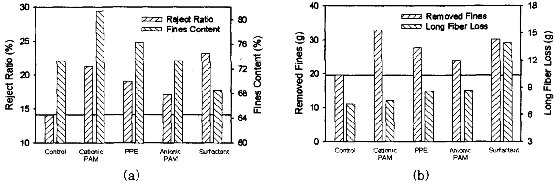
Fig. 5. Fines fractionation efficiency of OCC flotation in terms of several additives.
