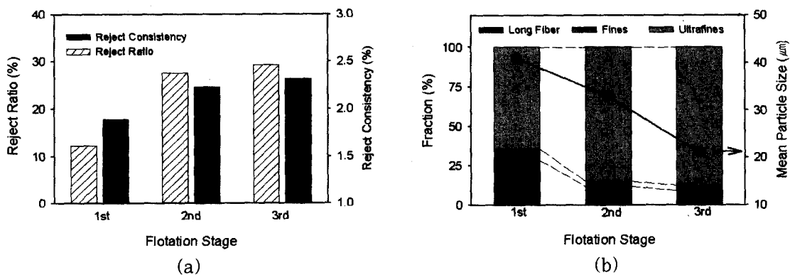
Fig. 2. The effect of flotation stages on fines fractionation of OCC.
