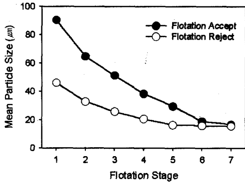
Fig. 3. The effect of flotation stages on mean particle size of fractionated fines.
