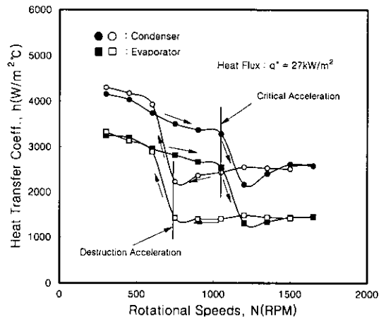
Fig. 8. Variation of heat transfer coefficient as a function of rotational speeds for a heat pipe with grooves.
