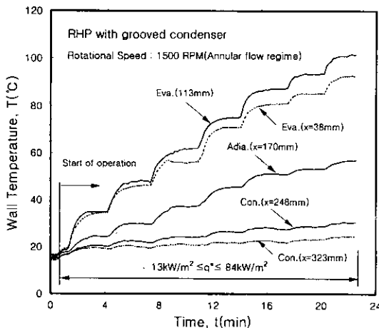
Fig. 7. Wall temperature variations with various heat flux for heat pipe with grooves at rotational speed of 1500RPM (Annular flow regime).
