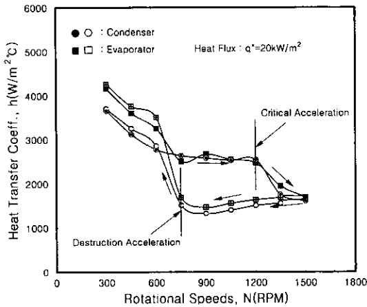
Fig. 9. Variation of heat transfer coefficient as a function of rotational speeds for a heat pipe with circular cross section.
