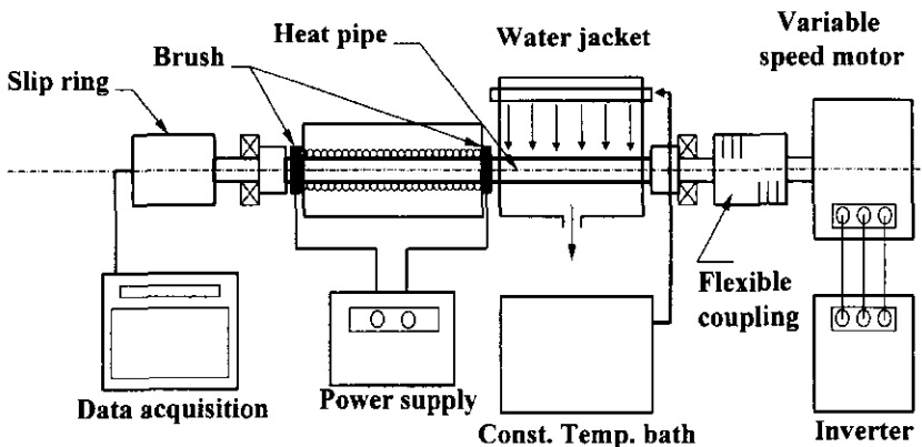
Fig. 3. Schematic diagram of the experimental apparatus for performance test of a rotating heat pipe.
