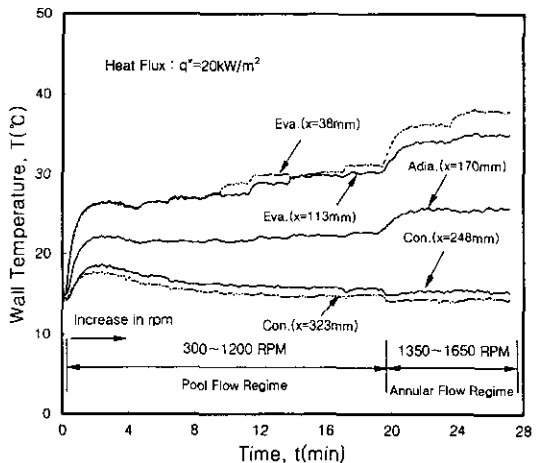
Fig. 5. Wall temperature variations with rotational speeds for heat pipe without groove at constant heat flux of 20 kW/m 2 .
