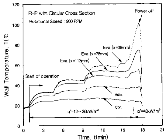
Fig. 11. Temperature rise due to local dry-out on the surface of evaporator caused by the deficit of condensate flow running for the evaporator, when heat flux was increased to 48 kW/m².
