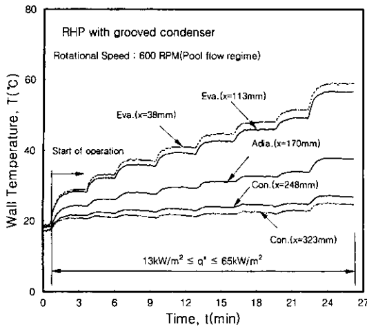
Fig. 6. Wall temperature variations with various heat flux for heat pipe with grooves at rotational speed of 600RPM (Pool flow regime).
