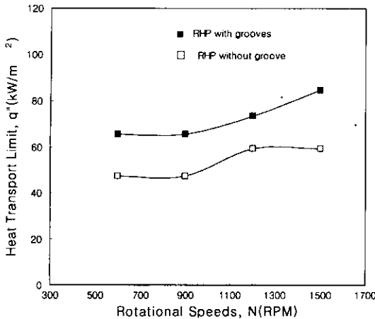
Fig. 12. Heat transport limitation along with rotational speeds for 2 types of heat pipes, uniform circular cross section and grooved condenser heat pipe.
