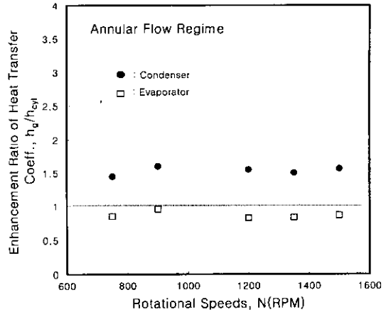
Fig. 10. The enhancement ratio of evaporator and condenser heat transfer coefficient for a heat pipe with grooves which are compared with the values of a circular cross section rotating heat pipe at annular regime.
