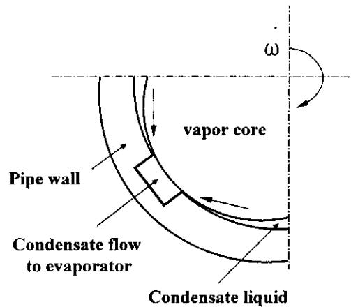
Fig. 1. Condensate flow in a rotating heat pipe with grooves.
