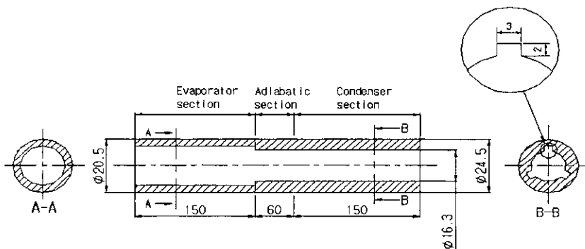
Fig. 2. Longitudinal cross section of a rotating heat pipe with grooves.
