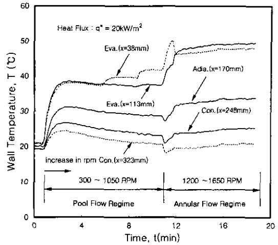
Fig. 4. Wall temperature variations with rotational speeds for heat pipe with grooves at constant heat flux of 20 kW/m 2 .
