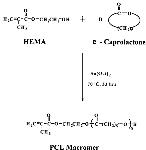
Scheme 2. Synthesis of PCL macromer.
