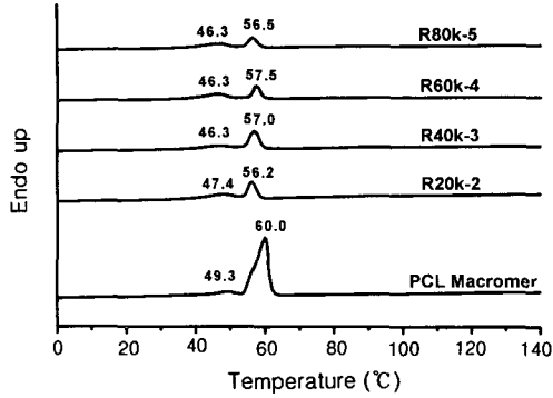
Figure 9. DSC 1st heating thermograms of R series (heating rate 20 °C/min).
