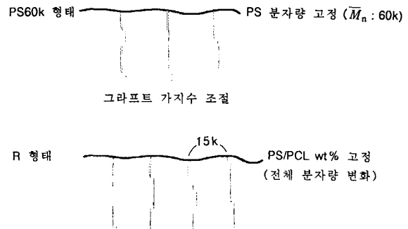
Scheme 1. Molecular structures of synthesized poly(styrene- g -caprolactone)s.
