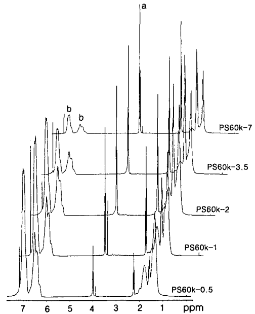
Figure 4. 1 H-NMR spectra of graft copolymers in CDCl 3 (PS60k series).
