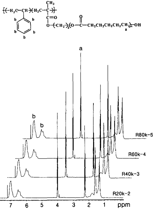
Figure 5. 1 H-NMR spectra of graft copolymers in CDCl 3 (R series).
