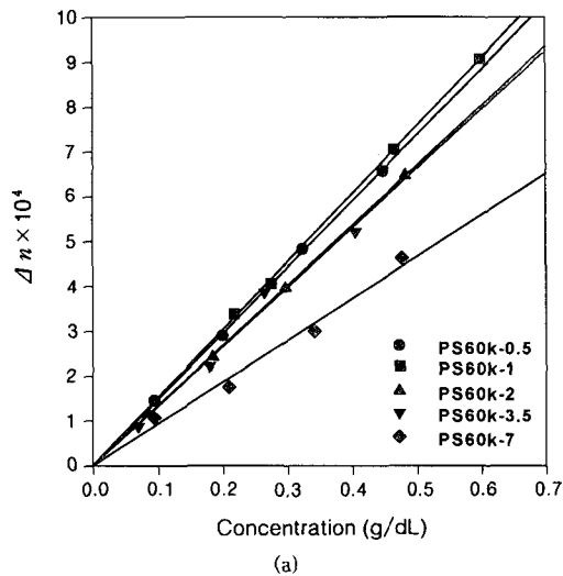
Figure 6. \Delta n vs. concentration plots of graft copolymers: (a) PS60k series and (b) R series.
