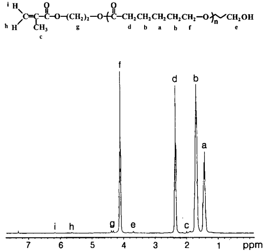
Figure 1. 300 MHz 1 H-NMR spectrum of PCL macromer in CDCl 3 .
