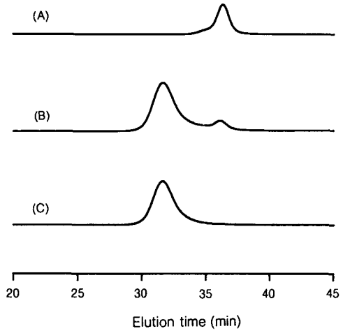
Figure 2. GPC traces of (A) PCL macromer, (B) PS- g -PCL before separation, and (C) PS- g -PCL after separation.
