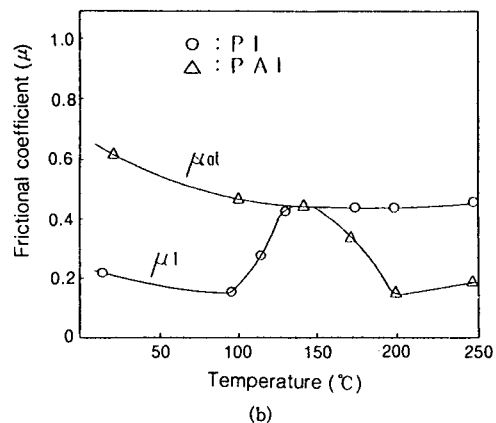
그림 4. Specific wear volume and frictional coefficient dependence on temp. (a) specific wear volume of polyimide and polyamideimide, (b) frictional coefficient of polyimide and polyamideimide.
