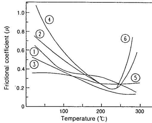
그림 3. Friction coefficient dependence on temperature of polyimide. ① : filler (BaSO 4 ), ② : 15% graphite, ③ : 15% MoS 2 , ④ : filler (CaCO 2 ) ⑤ : 15% PTFE ⑥ : 20% graphite.
