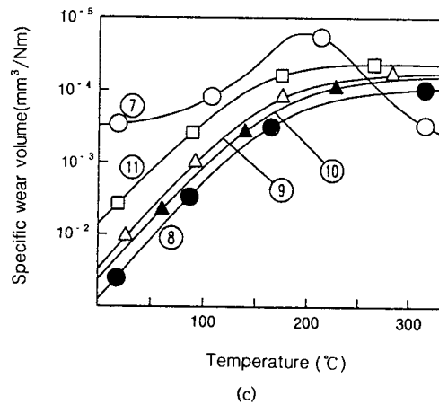
그림 2. Specific wear volume dependence on temperature of polyimide. Symbols and numbers are as indicated in Table 1.
