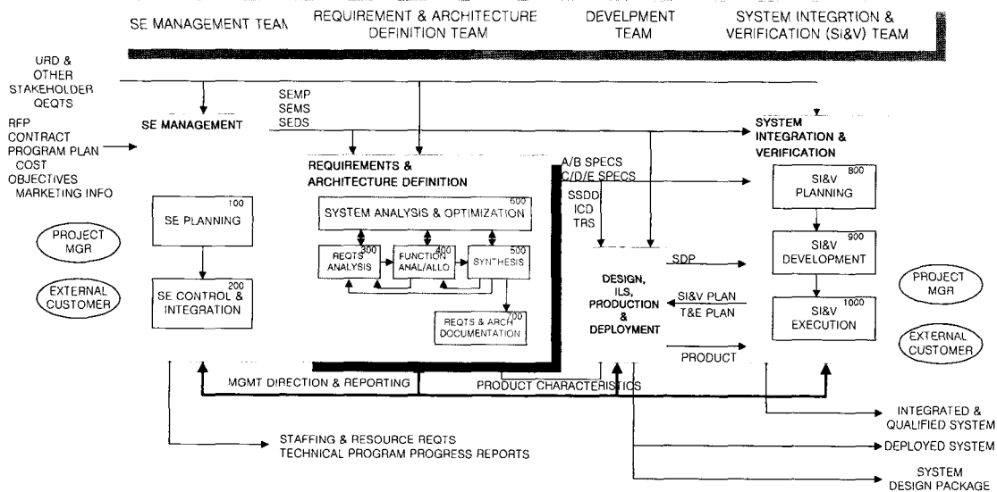
(그림 1) Systems Engineering Process
