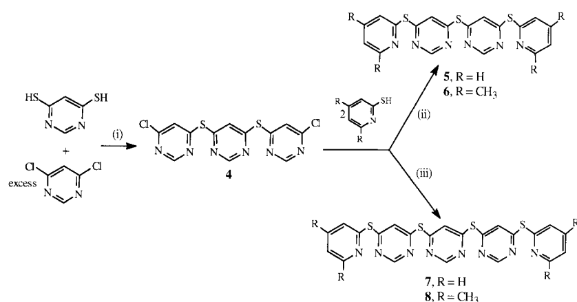
Scheme 1. Synthetic procedures for ligands for 3 \times 3 and 4 \times 4 molecular grids. (i) K_2CO_3/DMF (ii) K_2CO_3/acetone (iii) K_2CO_3/CH_2Cl_2 .
