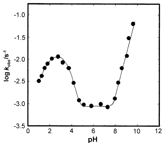
Figure 1. A plot of \log k_{\text{obs}} vs. pH for the hydrolysis of N -furoyl-2-phenylimidazole in \text{H}_2\text{O} at 40^\circ \text{C} , \mu = 0.5 \text{ M} with KCl.
