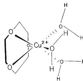
Figure 9. Schematic diagram of a Cu 2+ ion, located at site II* in an octahedral environment in TAPO-5, directly coordinating to three framework oxygens and three water molecules.
