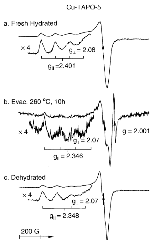
Figure 6. ESR spectra at 77 K of Cu-TAPO-5 (a) in fresh hydrated state, (b) evacuated at 260 °C for 10 h and (c) dehydrated by evacuation at 450 °C for 10 h, oxidation with dry oxygen at 450 °C for 5–10 h, and then evacuation at room temperature for 20 min.
