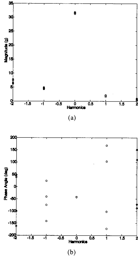
Fig. 5 (a) Magnitude response (b) Phase response. The excitation frequency is 2598 Hz
