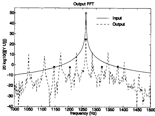
Fig. 3 The magnitude response of the input and output time series. The excitation frequency is 1262 Hz
