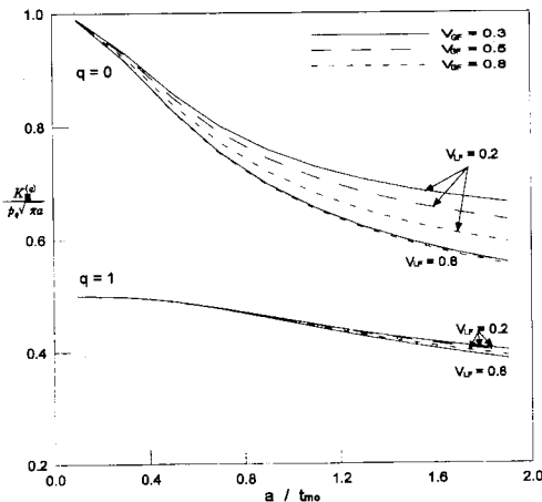
Fig. 5 Dimensionless mode III stress intensity factor for monolithic composites
