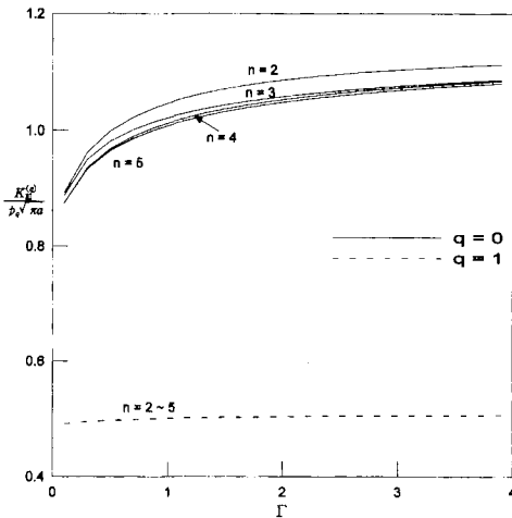
(a) a/t_0=1.0
