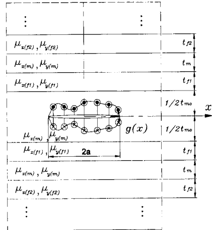
Fig. 6 Geometry of hybrid composites
