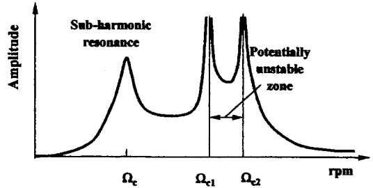
Fig. A-2 Vibratory characteristics of a simple rotor with stiffness asymmetry
