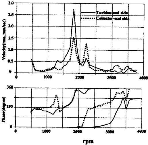
Fig. 6 2x vibration of bearing pedestals in z-direction
