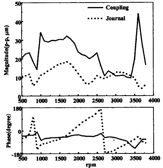
Fig. 3 1x vibration in z-direction: uncompensated
