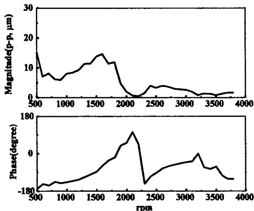
Fig. 9 2x vibration of journal in z-direction: uncompensated
