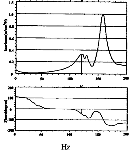
Fig. 7 Frequency response function of fixture
