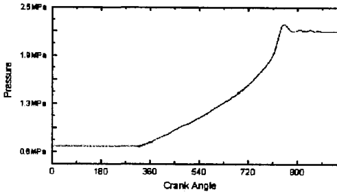
Fig. 8 Pressure pulsation in the discharge port
