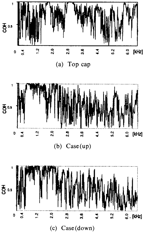
Fig. 10 Coherence of vibration and noise at top cap and case
