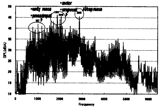
Fig. 18 Noise sources of main frequencies
