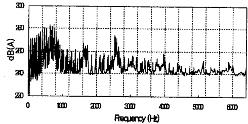
(a) Pressure pulsation
