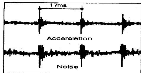
Fig. 4 Measured accelerometer and microphone time domain response
