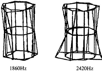
Fig. 16 Mode shape of case
