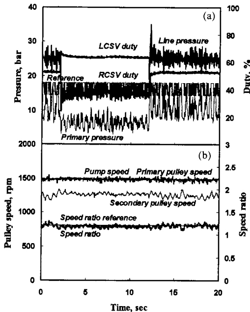
Fig. 18 Response for line pressure disturbance with fuzzy control
