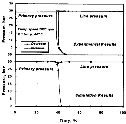
Fig. 5 RCV characteristics
