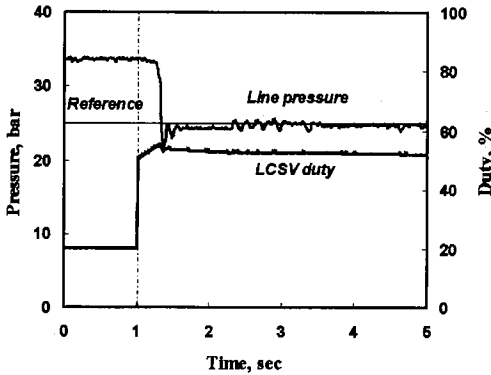
Fig. 11 Line pressure response for feedforward controller
