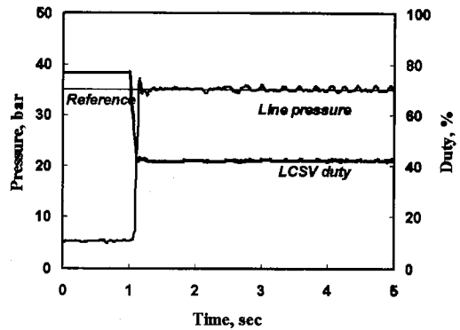
Fig. 7 Line pressure response of LRV
