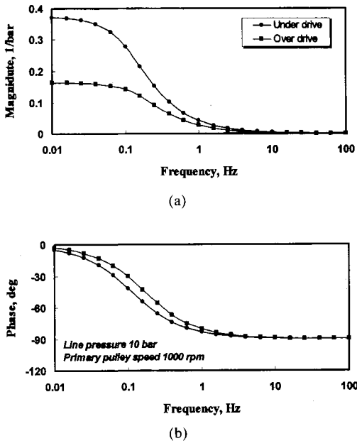
Fig. 3 Frequency response
