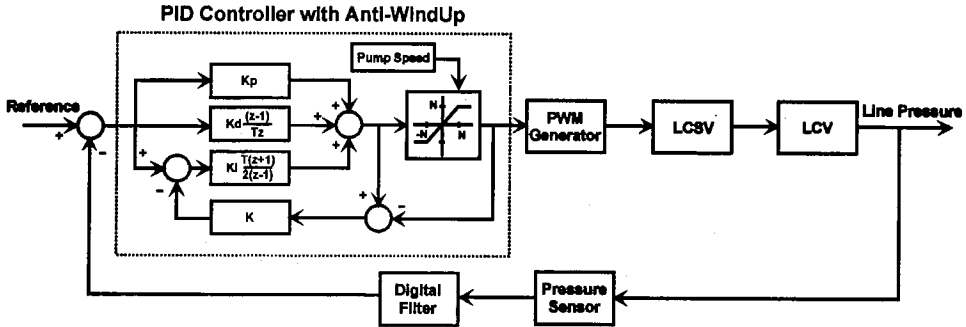
Fig. 6 Block diagram of low level control for line pressure
