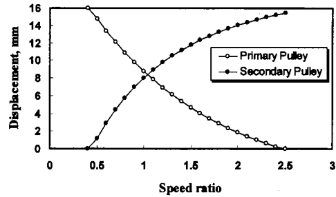
Fig. 2 Movable pulley displacement vs. speed ratio
