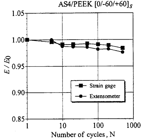
Fig. 6 Stiffness loss of [0/-60/60]_s AS4/PEEK laminate
