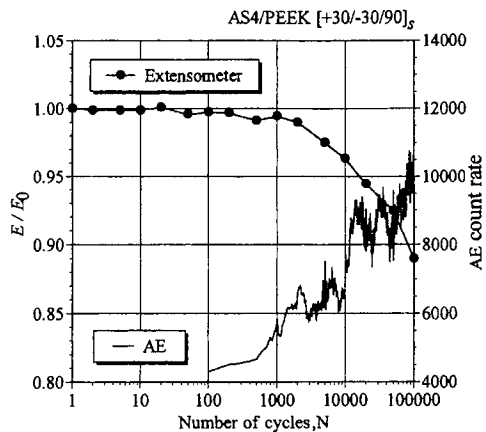
Fig. 11 Stiffness loss and AE count rate of [30/-30/90] s AS4/PEEK laminate
