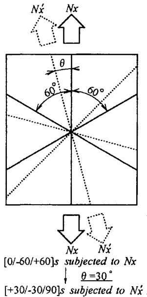
Fig. 1 Variation of tensile loading direction
