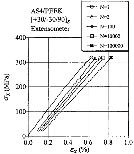
Fig. 10 Stress-strain curve of [30/-30/90] s AS4/PEEK laminate
