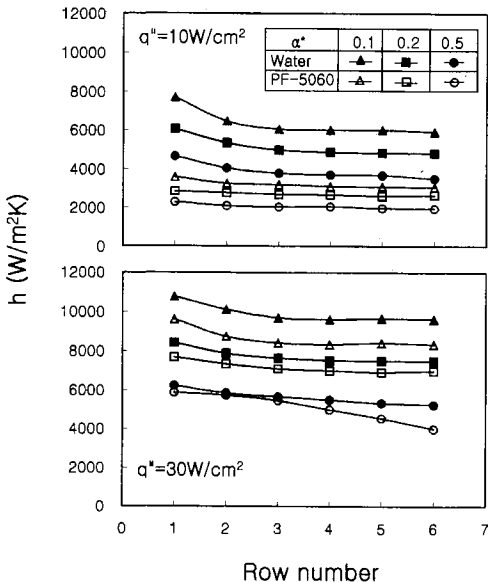
Fig. 4 Local heat transfer coefficient with respect to row number ( Re_{dh} = 15,000 )
