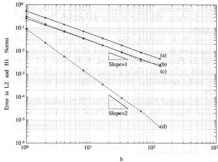
FIGURE 1. H^1 and L^2 errors with the h version.
