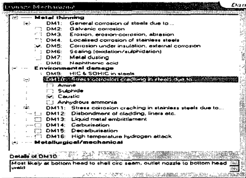
Fig. 8. Damage mechanisms considered in W-software.
