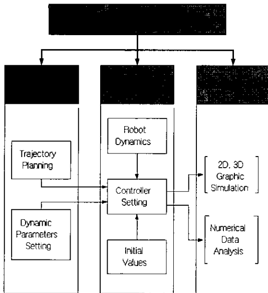
Fig. 1 The Structure of Off-Line Programming System
