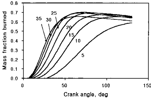
Fig. 2 Mass fraction burned vs. crank angle for spark timings
