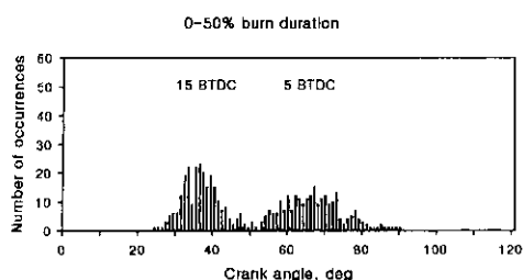
Fig. 11 Number of occurrences vs. crank angle for 0-50% burn duration at 5° BTDC and 15° BTDC spark timings
