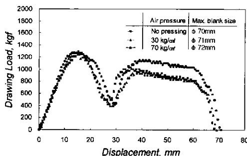
Fig. 7 Comparison of drawing load with increasing air pressure
