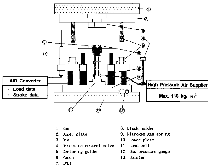
Fig. 2 Experimental setup of deep drawing process
