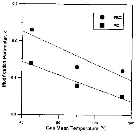
Fig. 8 Trends of modification parameters with variation of gas mean temperature
