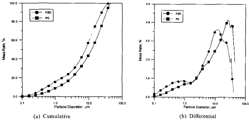
Fig. 4 Size distribution of fly-ashes from two coal combustion
