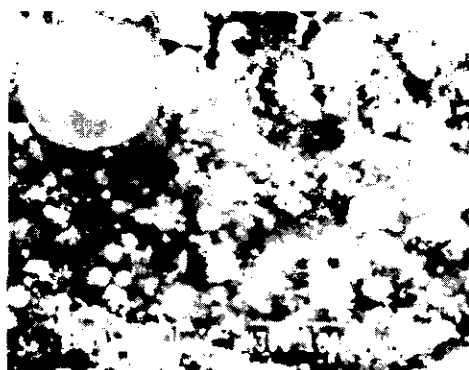
Fig. 3 Shape of fly-ash from pulverized coal combustion
