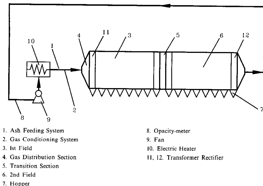
Fig. 1 Schematic diagram of pilot scale electrostatic precipitator
