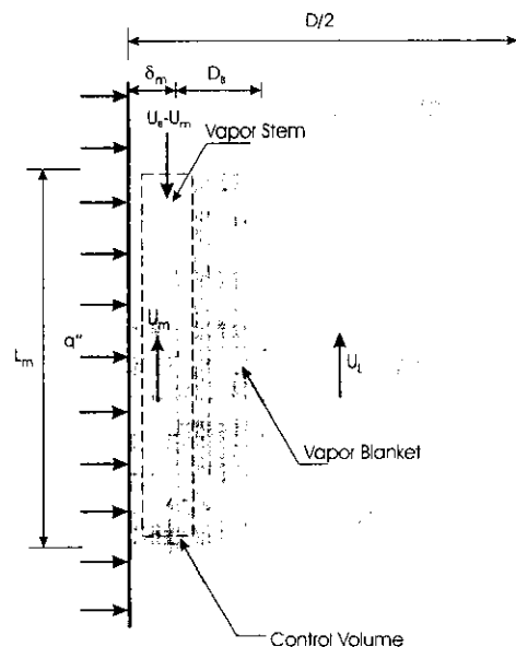
Fig. 1 Schematic of control volume for the sublayer dryout
