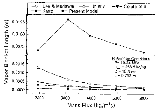
Fig. 6 Vapor blanket length as a function of mass flux
