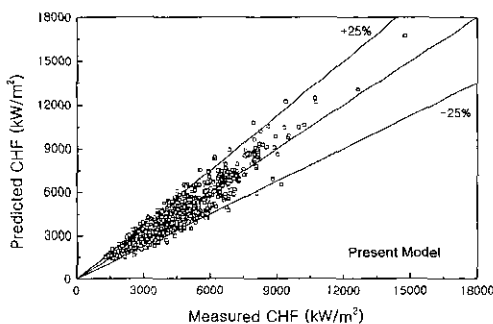
Fig. 5 Comparison of the predicted CHF using the present model with the experimental data
